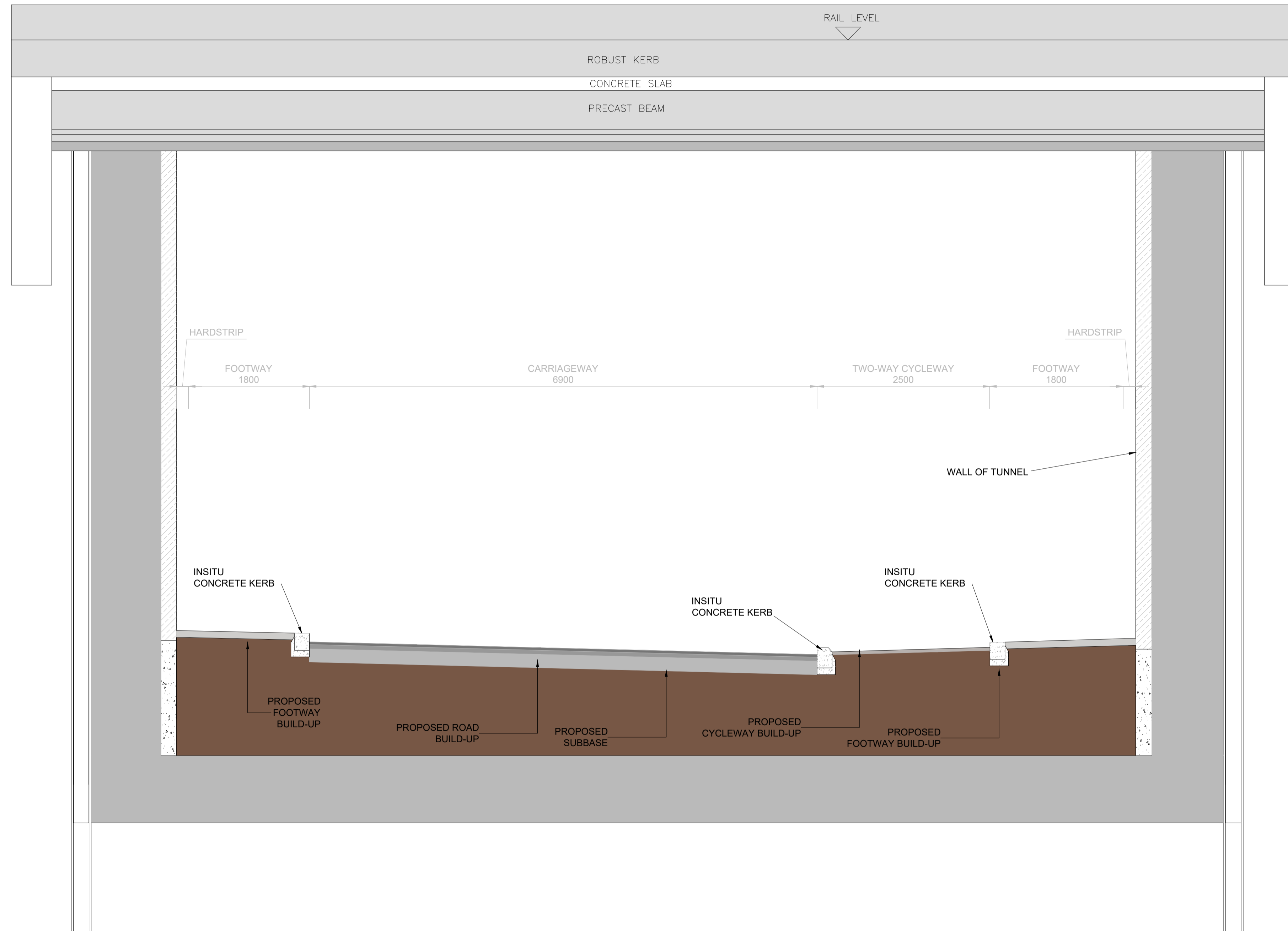
TYPICAL SECTION C-C SCALE 1:40
